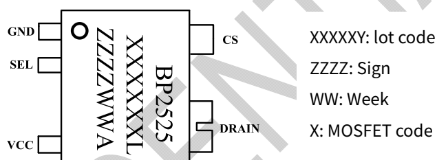
Figure 2. Pin configuration
